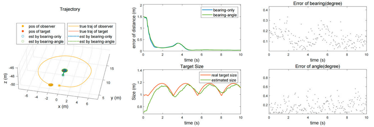
(b) Estimation results when \sigma_l = 0.01 and the other parameters are the same as those in Section 8.3.
