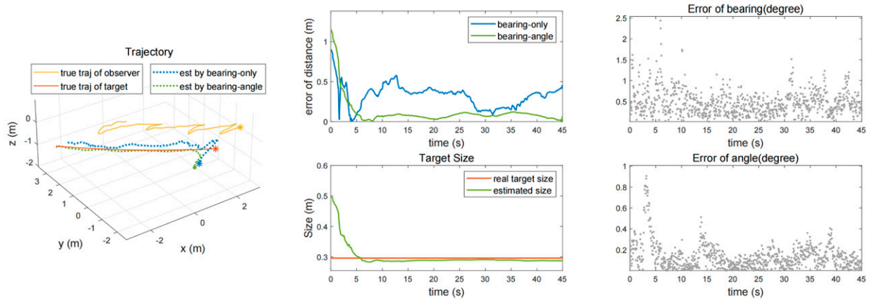
(b) Case 2: The observer moves close or far from the target periodically. The bearing-angle approach performs effectively, but the bearing-only approach works unstably.
