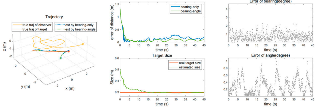
(a) Case 1: The observer moves around the target. Both the bearing-only and bearing-angle approaches work well.
