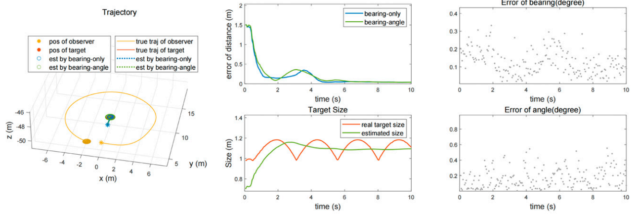
(a) Estimation results when \sigma_l = 10^{-4} and the other parameters are the same as those in Section 8.3.
