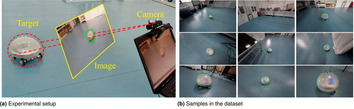
Figure 10. The setup of the experiments based on a hand-held camera. (a) Experimental setup, (b) Samples in the dataset.
