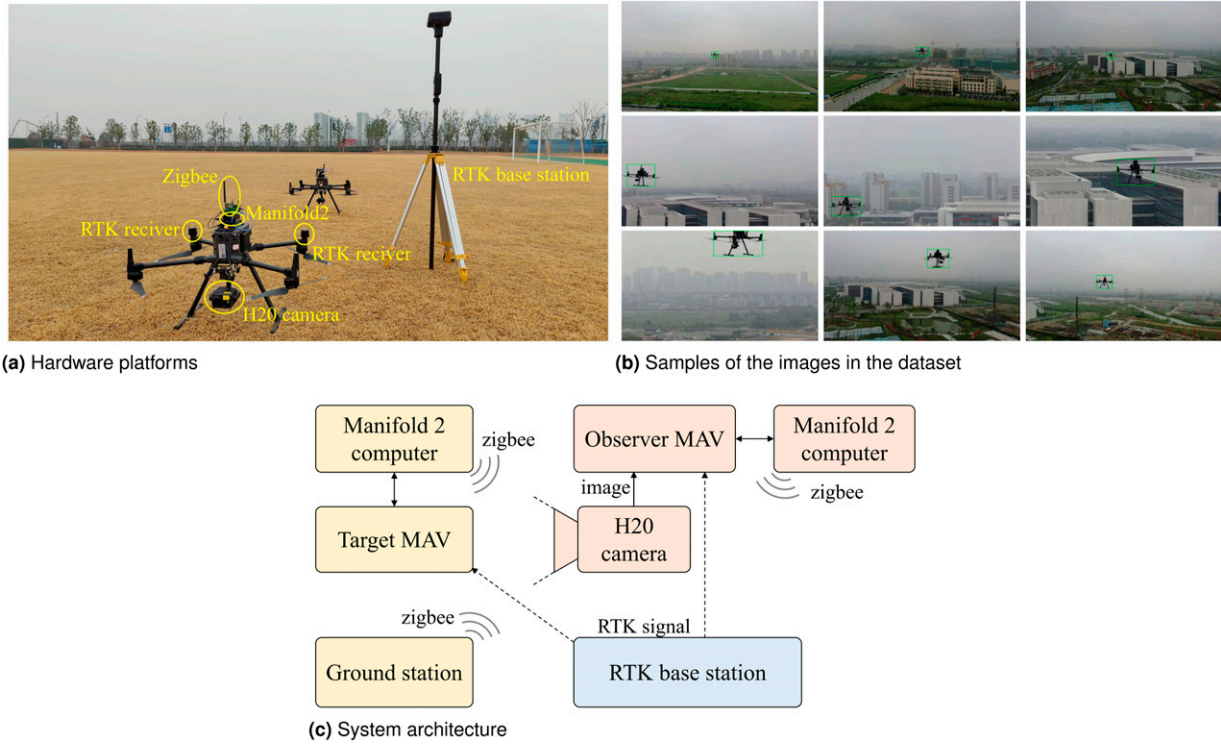
Figure 12. The setup of the MAV-following-MAV experiment. (a) Hardware platforms, (b) Samples of the images in the dataset, (c) System architecture.
